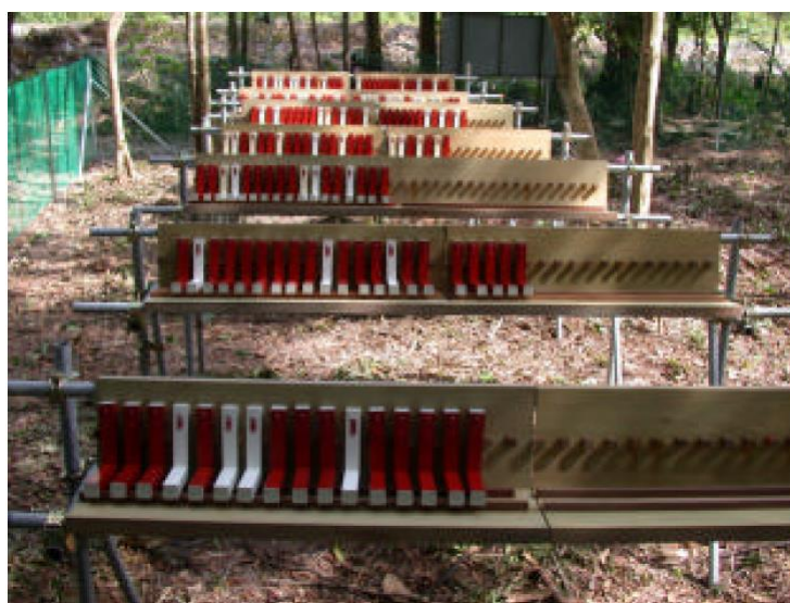
Figure 2. L-joints exposed in Malaysia. Photo: DTI 2005.
